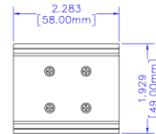
Rail piece
